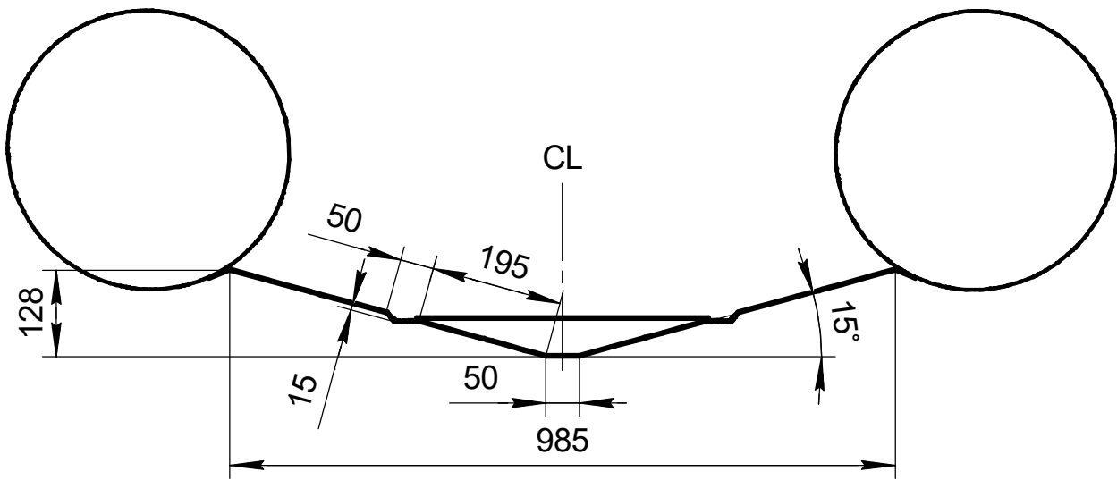
Section B
