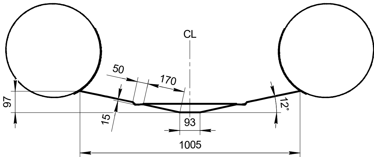
Section A
