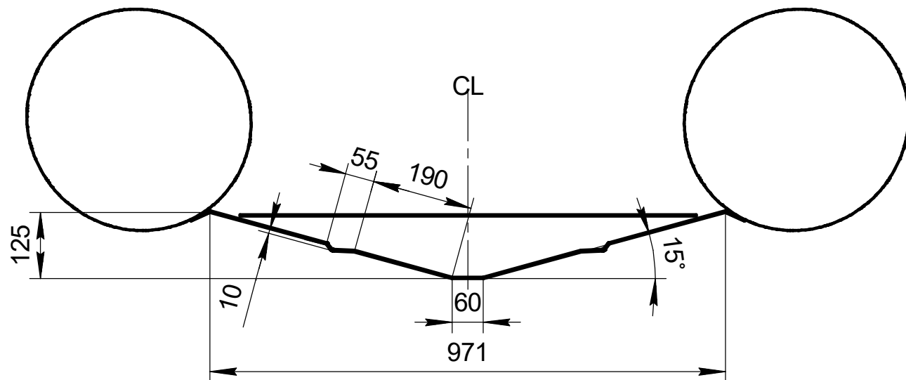
Section B
