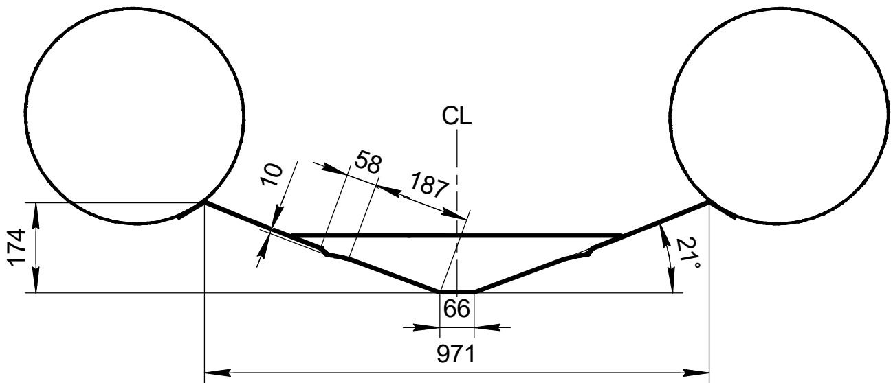
Section B
