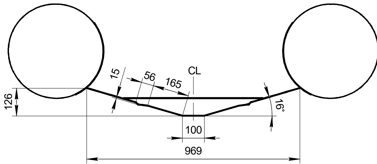
Section A
