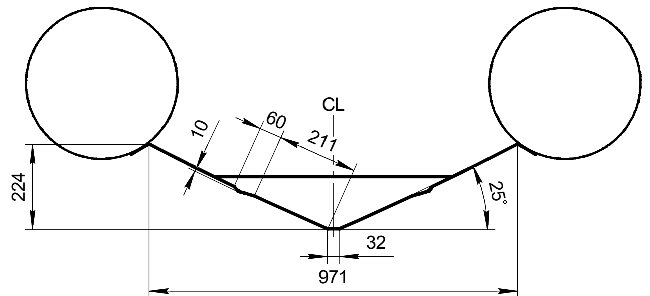
Section C
